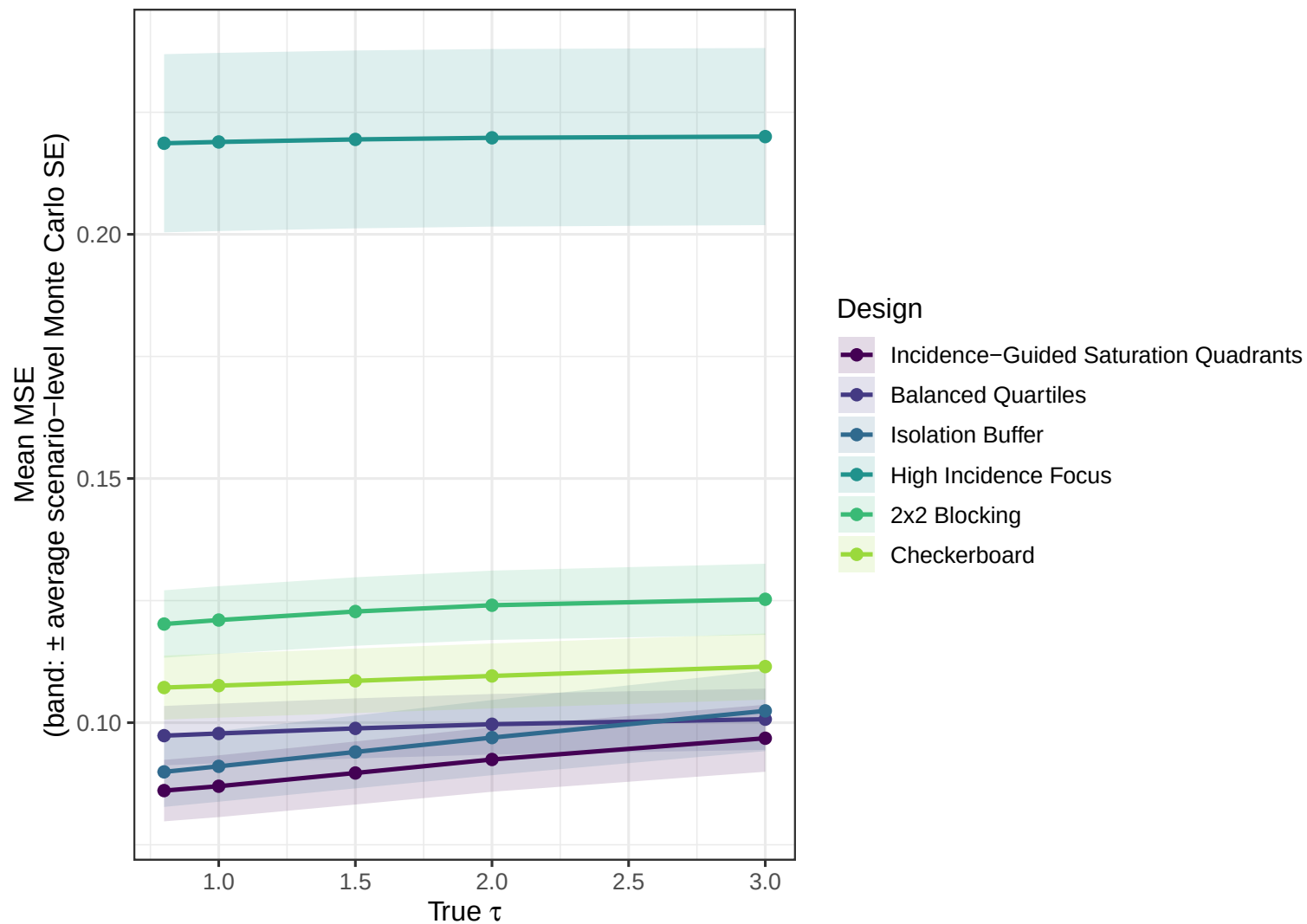
MSE vs. True \tau by Design
