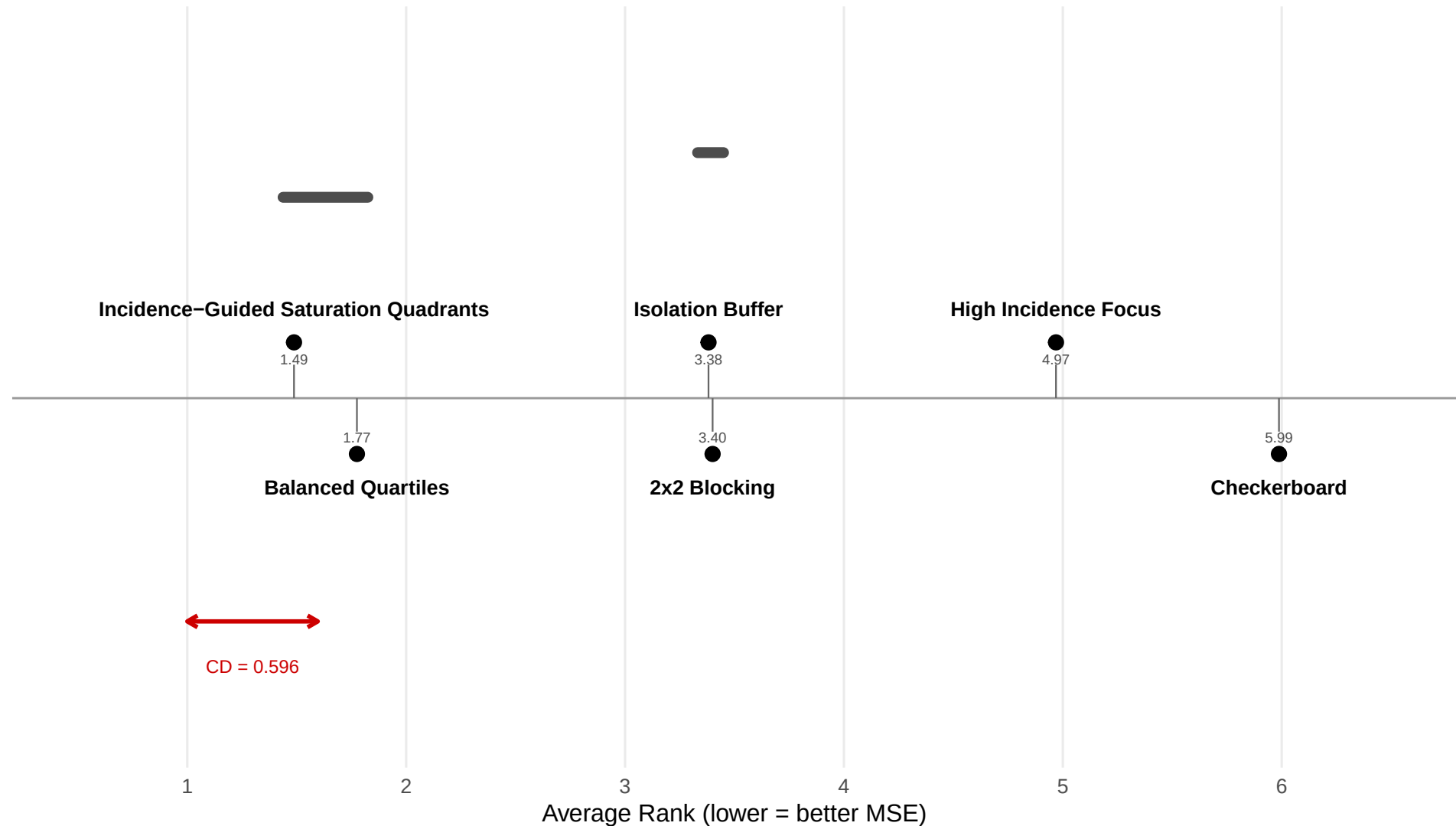
Critical Difference Diagram (6 designs, rook, tau=1.0)
