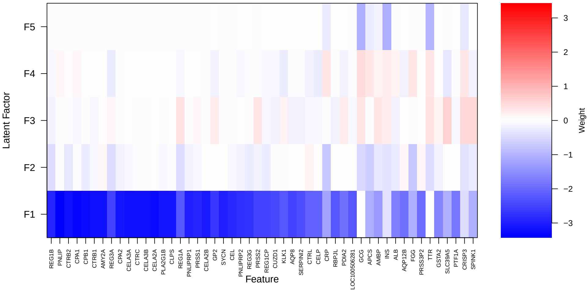
Figure 4: GEP Feature Weights (Top 50 Features) (CPTAC)
