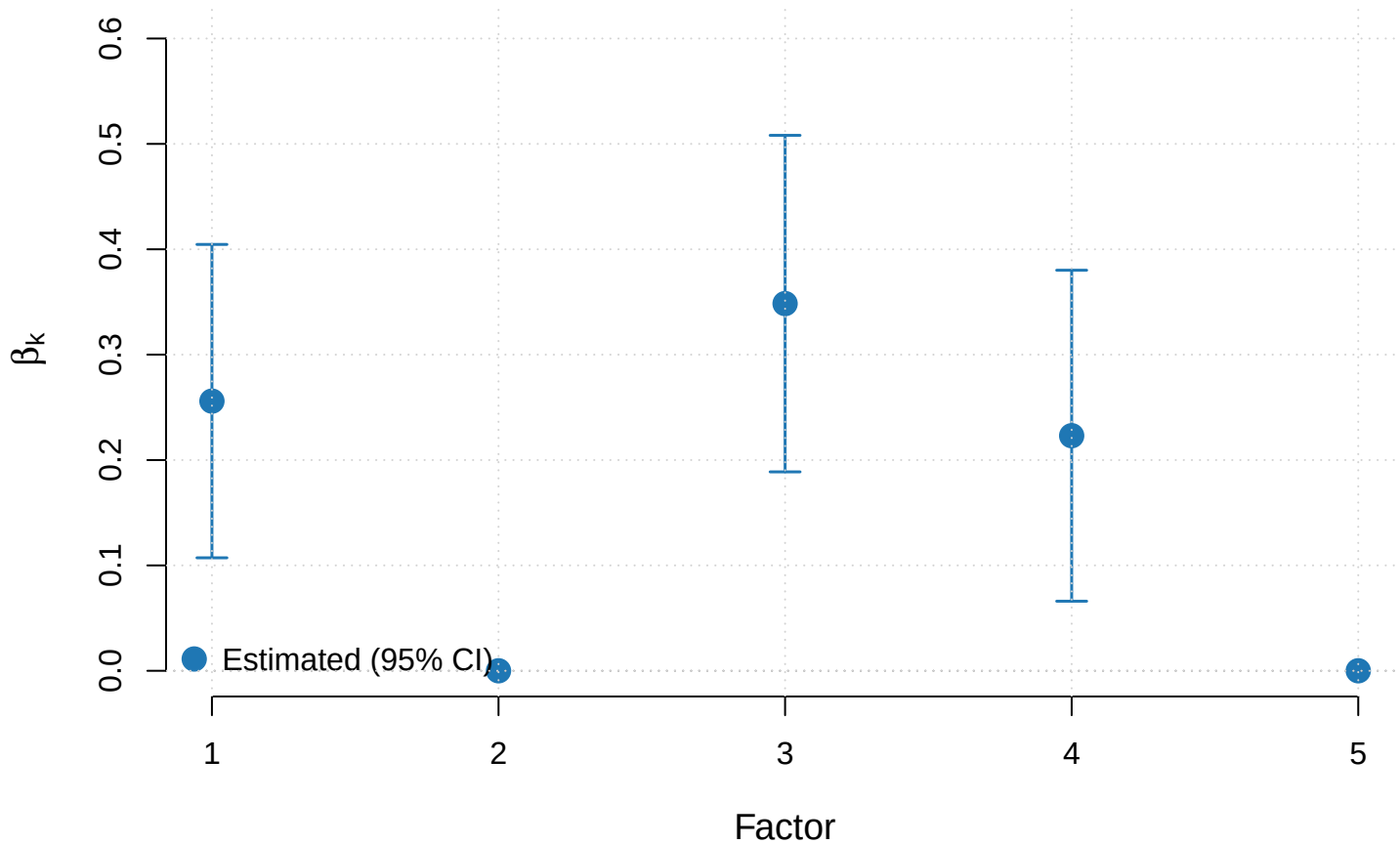
Figure 3: Estimated Survival Coefficients (95% CI) (Puleo_array)
