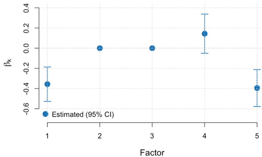
Figure 3: Estimated Survival Coefficients (95% CI) (PACA_AU_seq)
