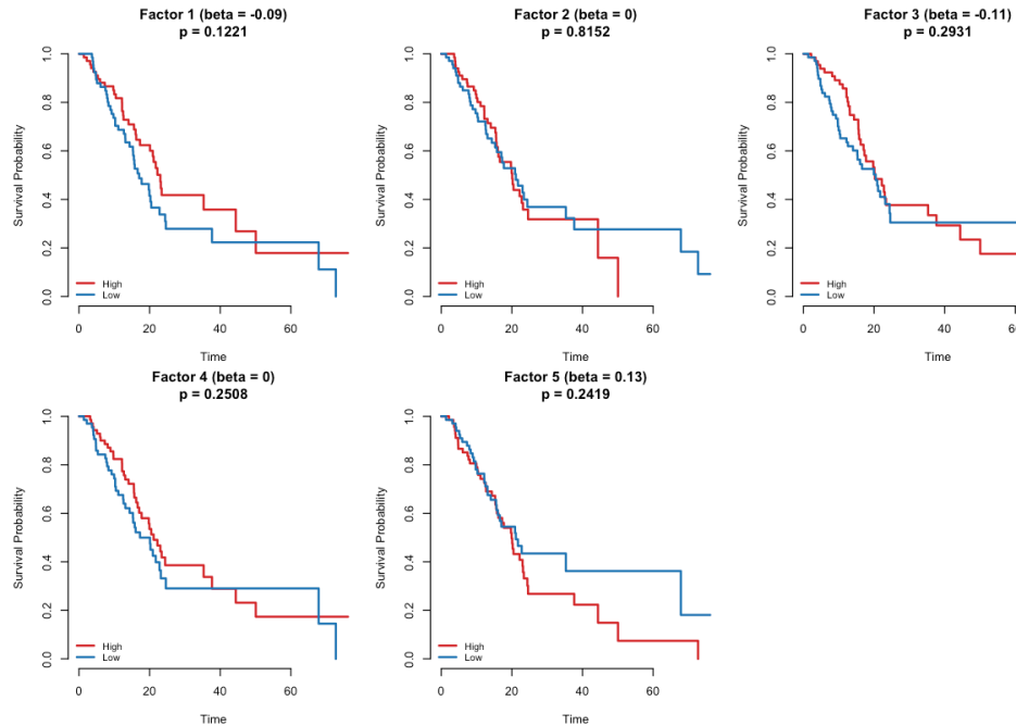
Figure 5: TCGA PAAD Kaplan-Meier
