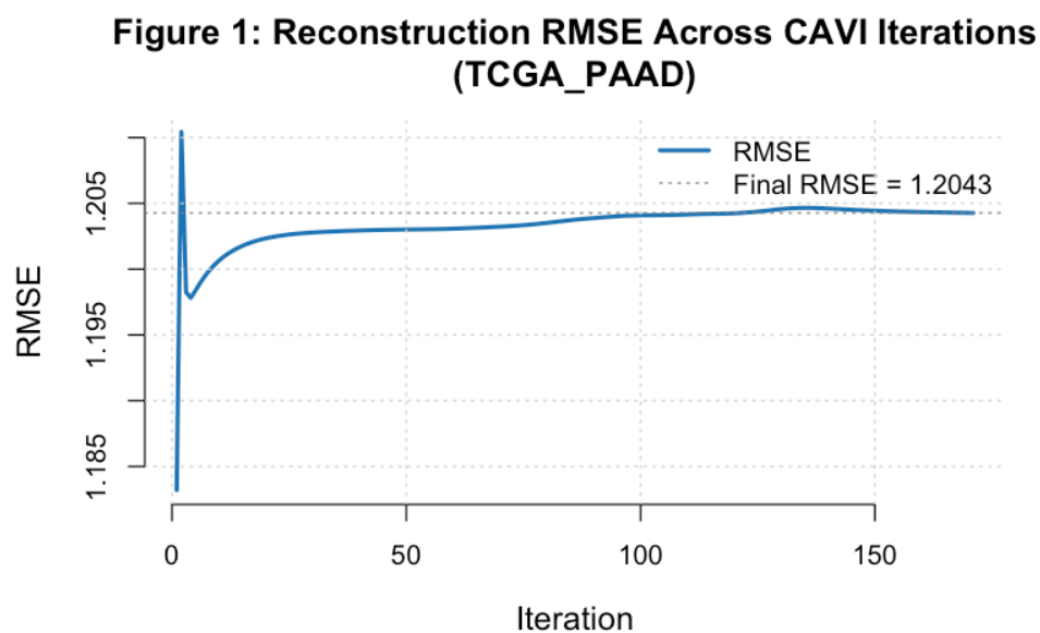
Figure 1: TCGA PAAD RMSE trace
