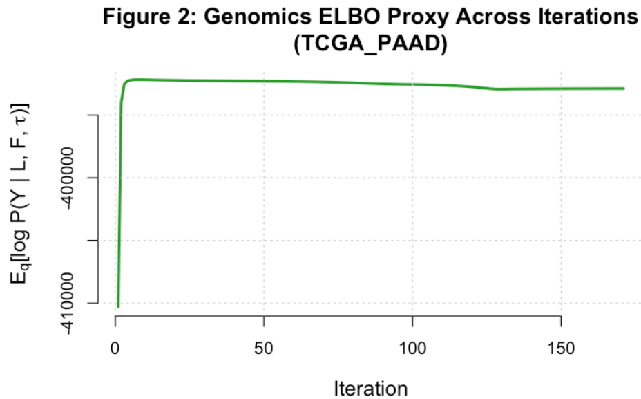
Figure 2: TCGA PAAD ELBO trace
