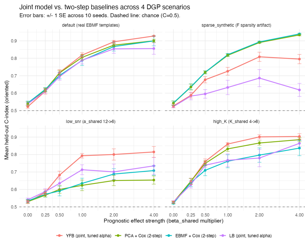
Figure 1: Each of the 4 panels is a different simulation design ( default = realistic factor-loading templates; sparse_synthetic = an artificial exact-sparse stress test; low_snr = weakened shared genomic signal; high_K = more shared latent factors ) – the panels are not different models. Within every panel, the x-axis is prognostic effect strength and the 4 colored lines are the models being compared: YFB (recommended, joint) and LB (the other joint variant) against two two-step baselines, PCA+Cox and EBMF+Cox. YFB pulls ahead of both two-step baselines as signal strength increases in 3 of 4 panels, with the gap widening through the highest signal level tested; the one reversal (sparse_synthetic) is the known factor-collapse artifact noted above, not a general failure of the joint approach.
