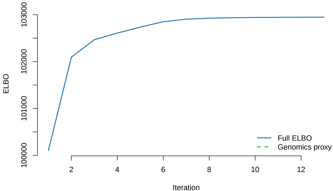
ELBO Convergence Trace
