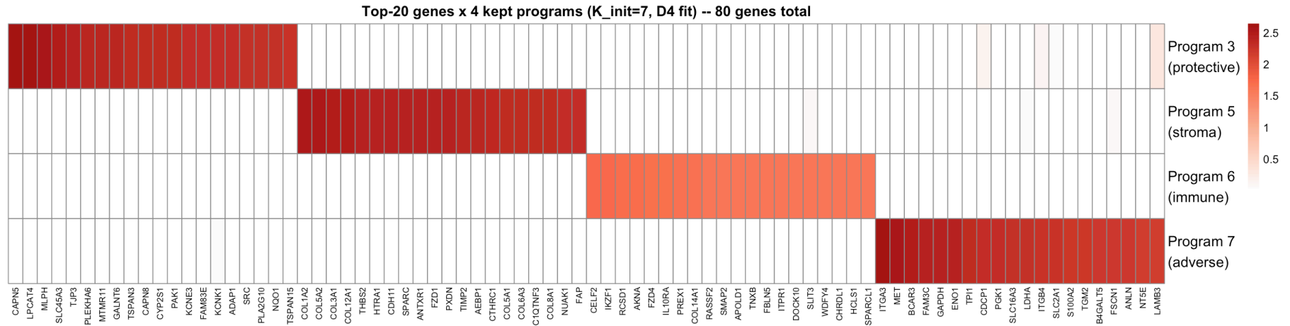
Figure 4: Figure. Top-20 genes by loading weight for each of K_{\text{init}} = 7 's 4 kept factors (the other 3, fully pruned, are omitted), rows = programs, columns = genes. Weights are non-negative (point-exponential prior); the block-diagonal structure means each program's top genes carry near-zero weight in the other 3.
