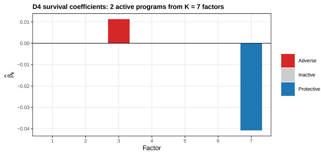
Figure 2: Posterior mean survival coefficients for D4 (YFB DeSurv-aligned, K = 7 ). Red bars = adverse programs (positive beta-hat, high loading predicts worse survival); blue bars = protective (negative beta-hat); grey = inactive factors shrunk to near-zero by the empirical Bayes prior. Only Factors 3 and 7 survive shrinkage; the remaining five factors capture expression variation that is not prognostically informative in the training cohort.
