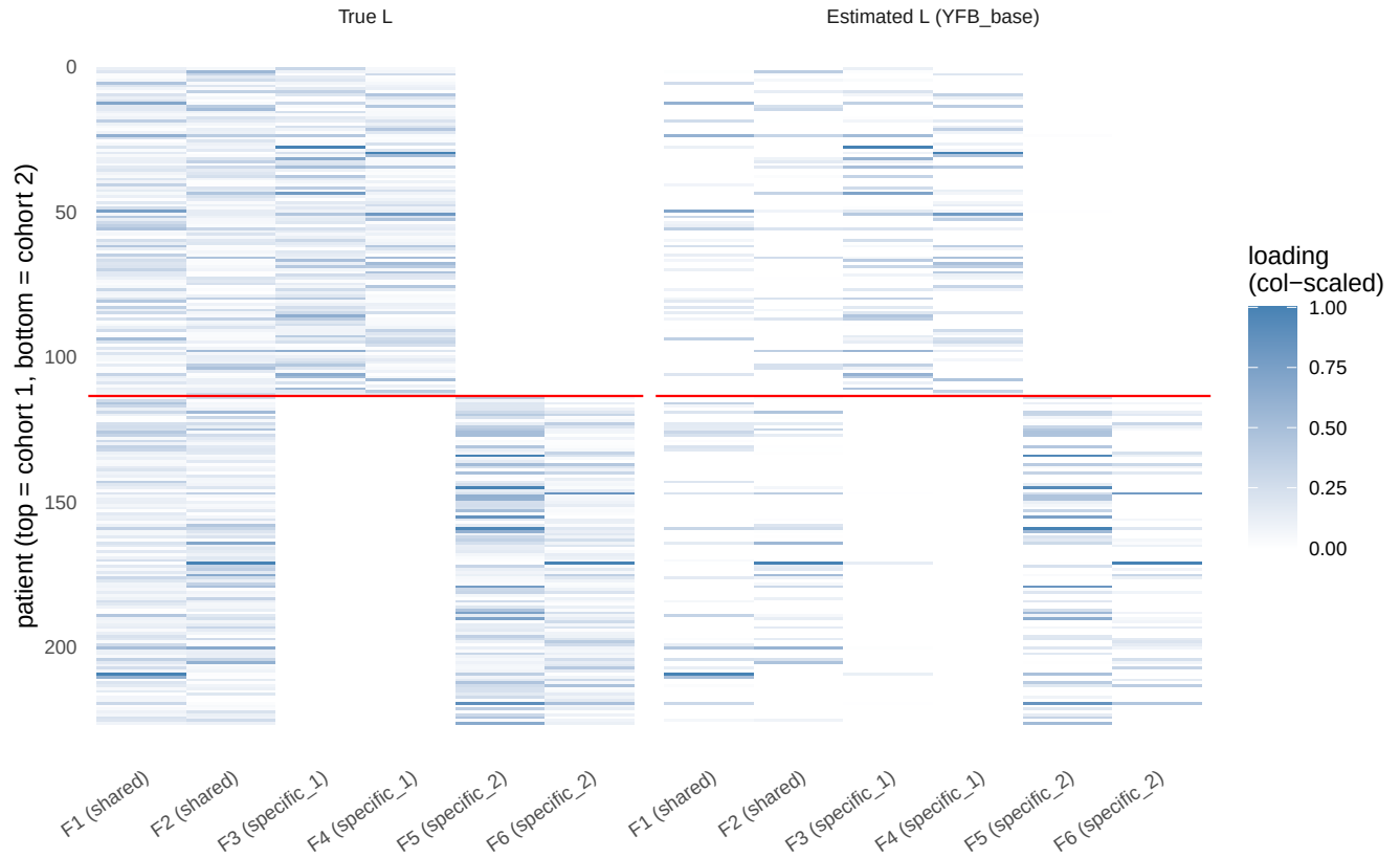
Figure 1: Patient loadings in the hybrid scenario (seed 1, training patients grouped by cohort; red line = cohort boundary). Left: true loadings L . Right: estimated loadings from YFB_base (no cohort indicator), with columns reordered to the matched true factors. Each column is scaled to its own maximum so structure is comparable. Shared factors (F1-F2) load across BOTH cohorts; cohort-1-specific factors (F3-F4) light up only the top block and cohort-2-specific factors (F5-F6) only the bottom block. The estimate reproduces the true block-sparse pattern — the model identifies which factors are shared and which are cohort-private without any indicator columns.
