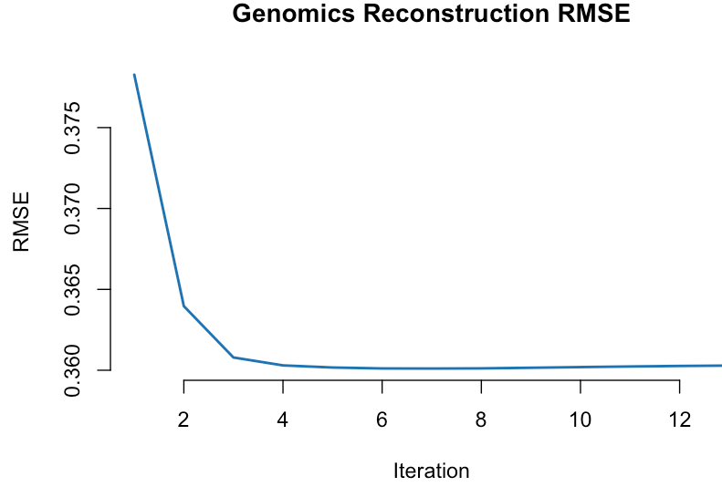
Figure 5: Genomics reconstruction RMSE vs. CAVI iteration ( point_normal ). The sharp initial drop reflects SVD initialisation; the plateau indicates convergence. Final RMSE is consistent with the synthetic noise level.
