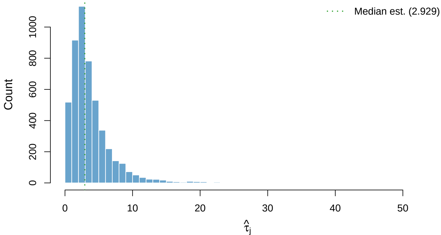
Figure 8: Estimated Feature-Specific Noise Precision (PACA_AU_seq)
