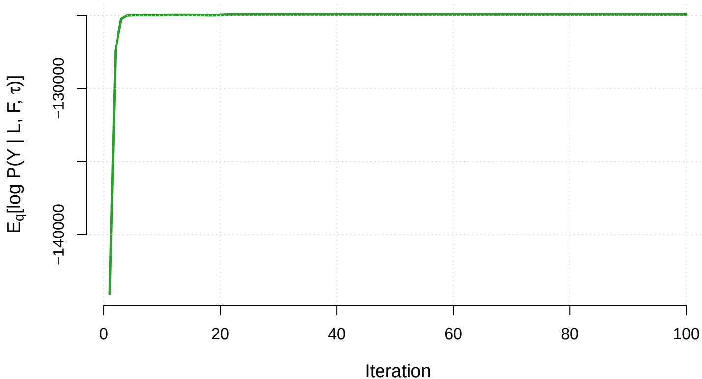
Figure 2: Genomics ELBO Proxy Across Iterations
