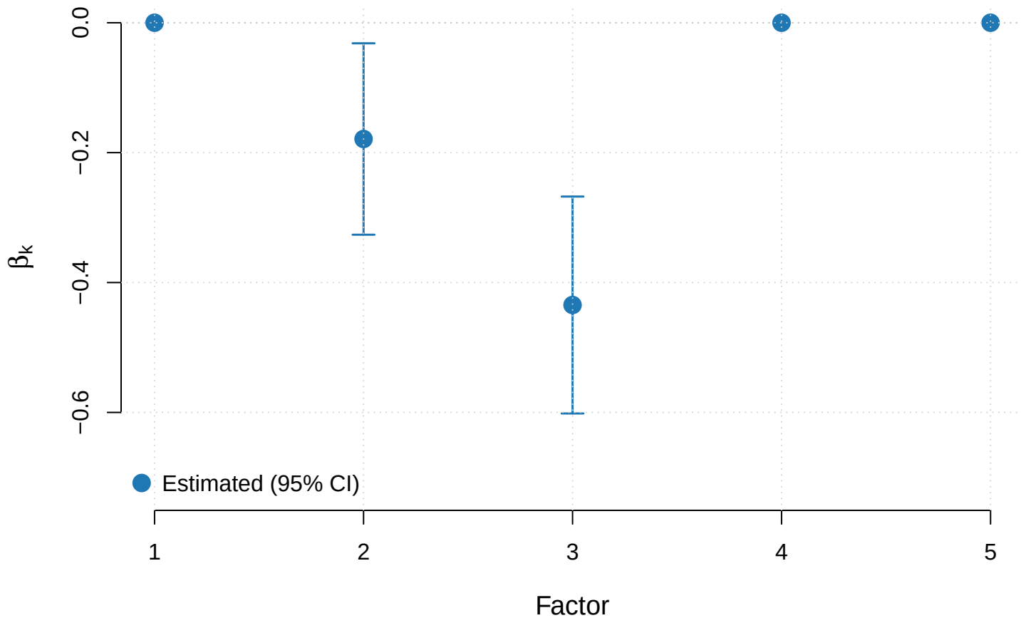
Figure 3: Estimated Survival Coefficients (95% CI) (CPTAC)
