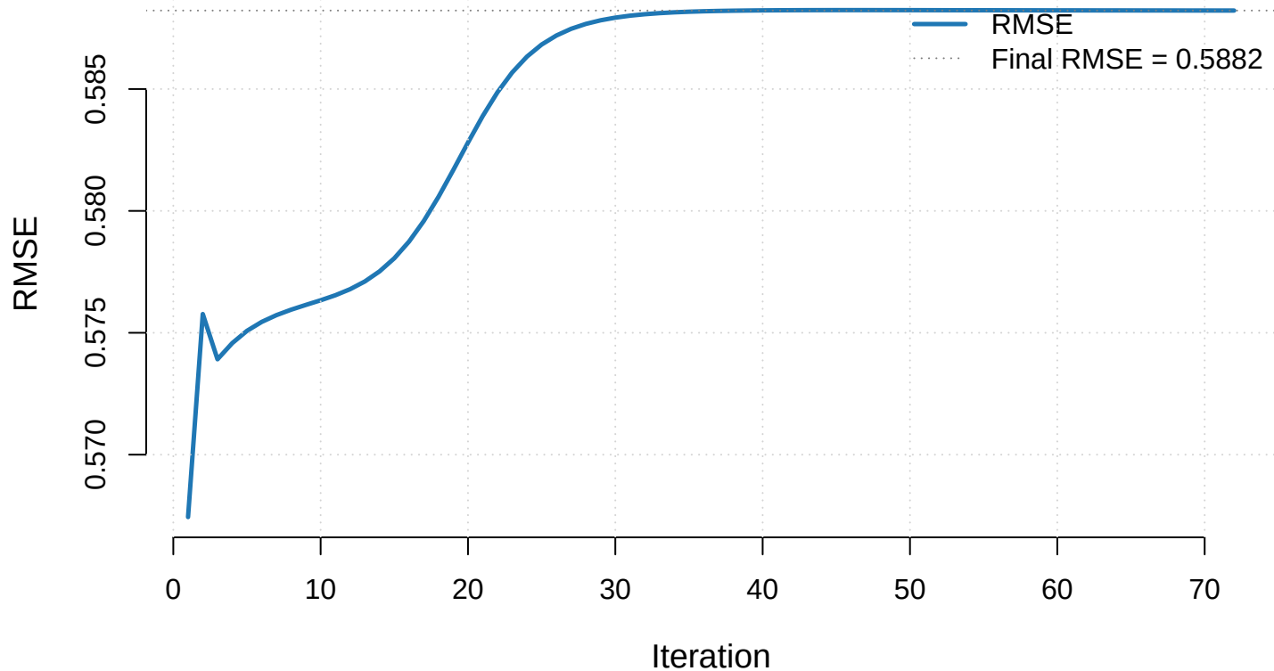
Figure 1: Reconstruction RMSE Across CAVI Iterations (Puleo_array)
