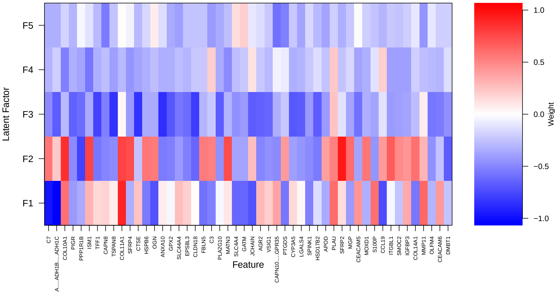
Figure 4: GEP Feature Weights (Top 50 Features) (Puleo_array)
