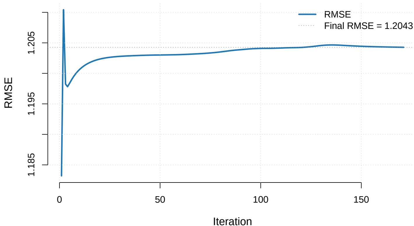
Figure 1: Reconstruction RMSE Across CAVI Iterations (TCGA_PAAD)
