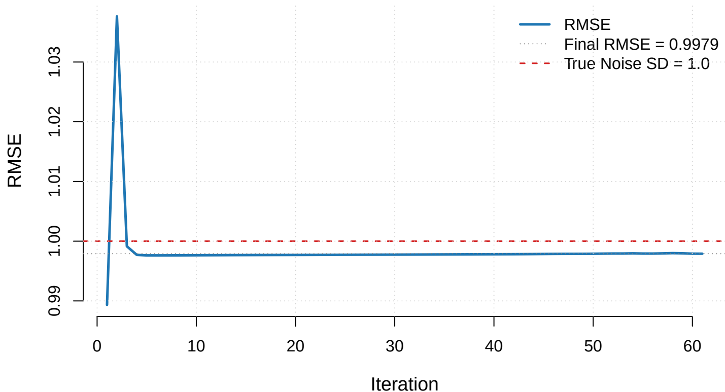
Figure 1: Reconstruction RMSE Across CAVI Iterations (Synthetic (n=250, p=1000, K=5))
