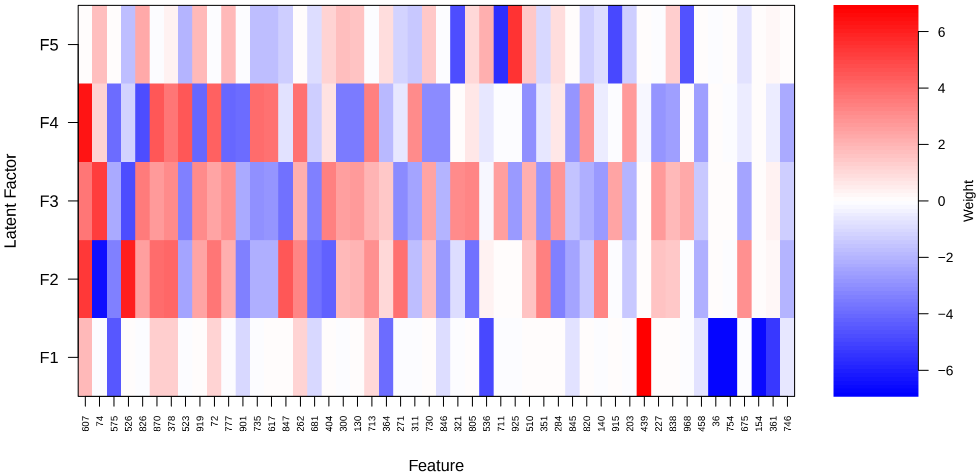
Figure 4: GEP Feature Weights (Top 50 Features) (Synthetic (n=250, p=1000, K=5))
