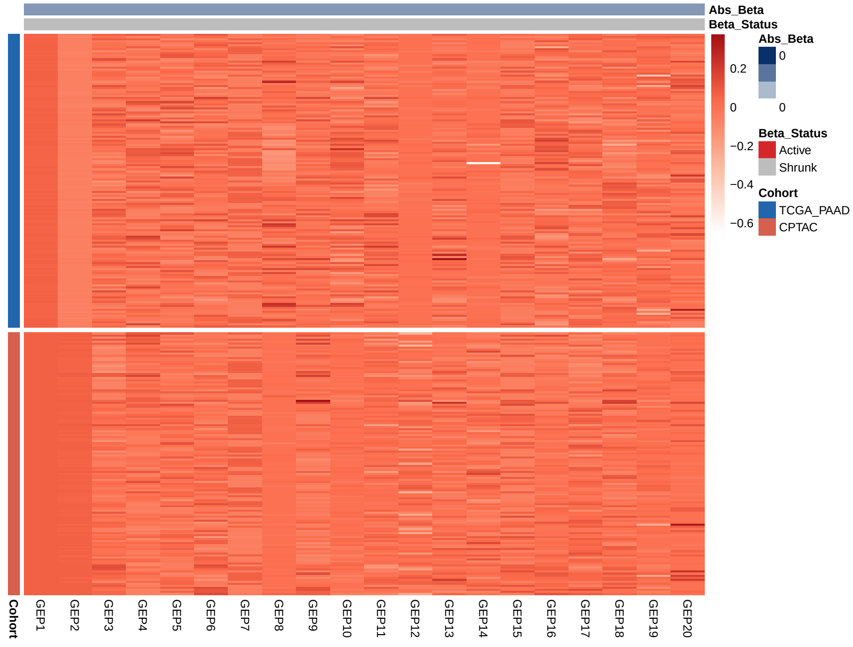
L-loading heatmap (samples by cohort) | n=273, K=20, |b|>0.05 marks 'Active'
