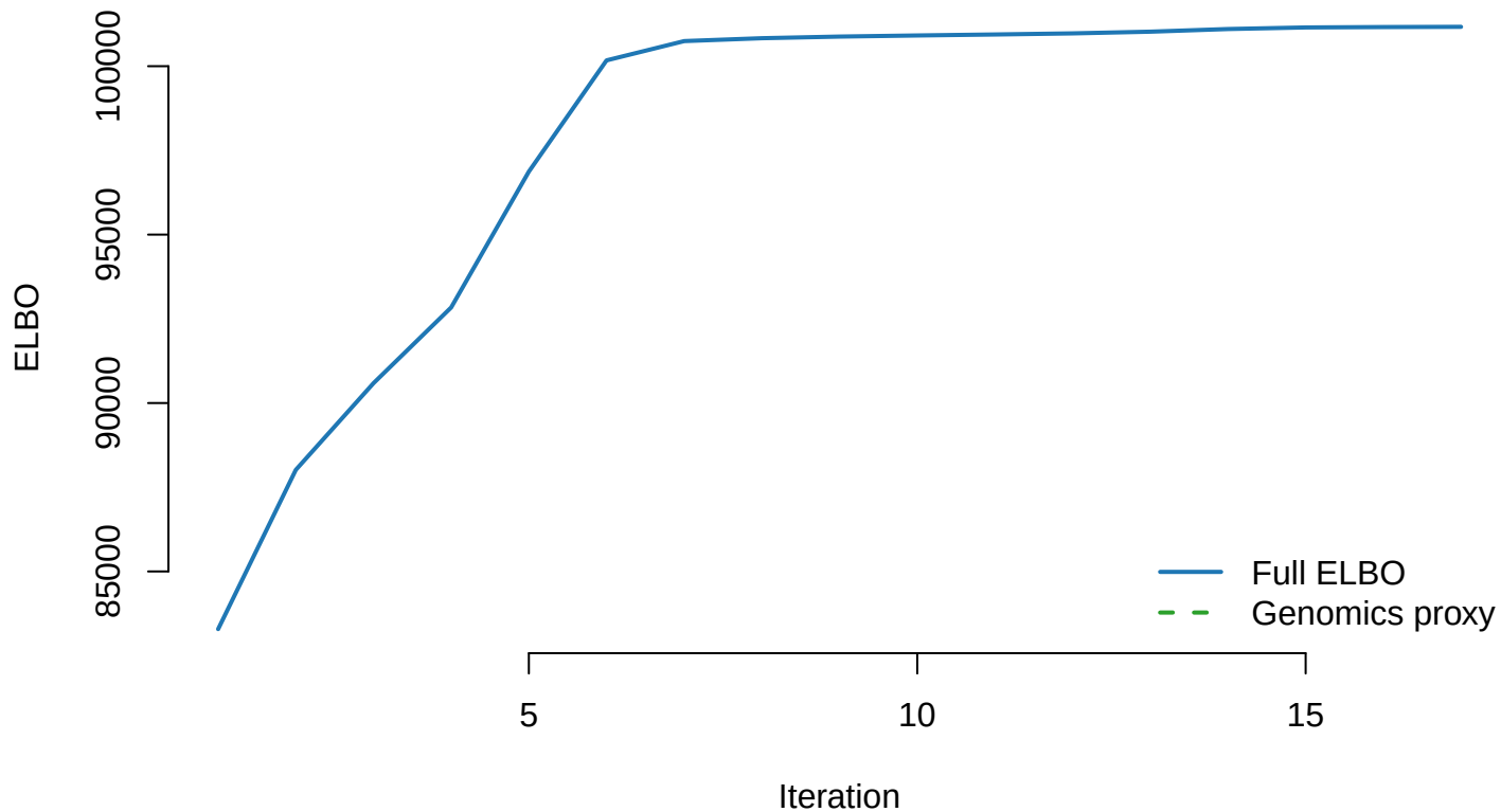
ELBO Convergence Trace
