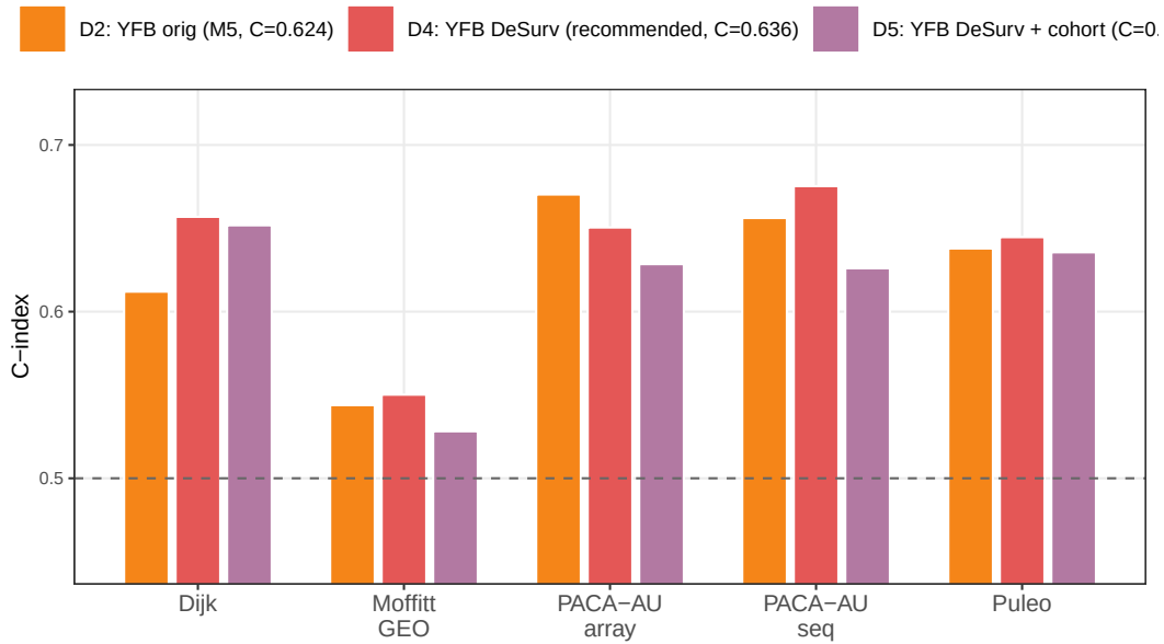
Figure 1: Per-cohort external concordance index for the three YFB configurations: D2 (original M5 baseline), D4 (DeSurv-aligned, recommended), and D5 (DeSurv-aligned + cohort indicator). Dashed line = chance ( C = 0.5 ). DeSurv selection (D4) improves over the baseline in 4 of 5 cohorts; the cohort indicator (D5) consistently reduces performance, with the largest regressions in PACA-AU-seq and PACA-AU-array.
