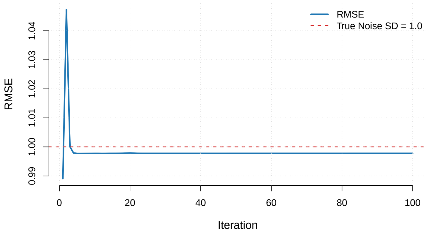
Figure 1: Reconstruction RMSE Across CAVI Iterations
