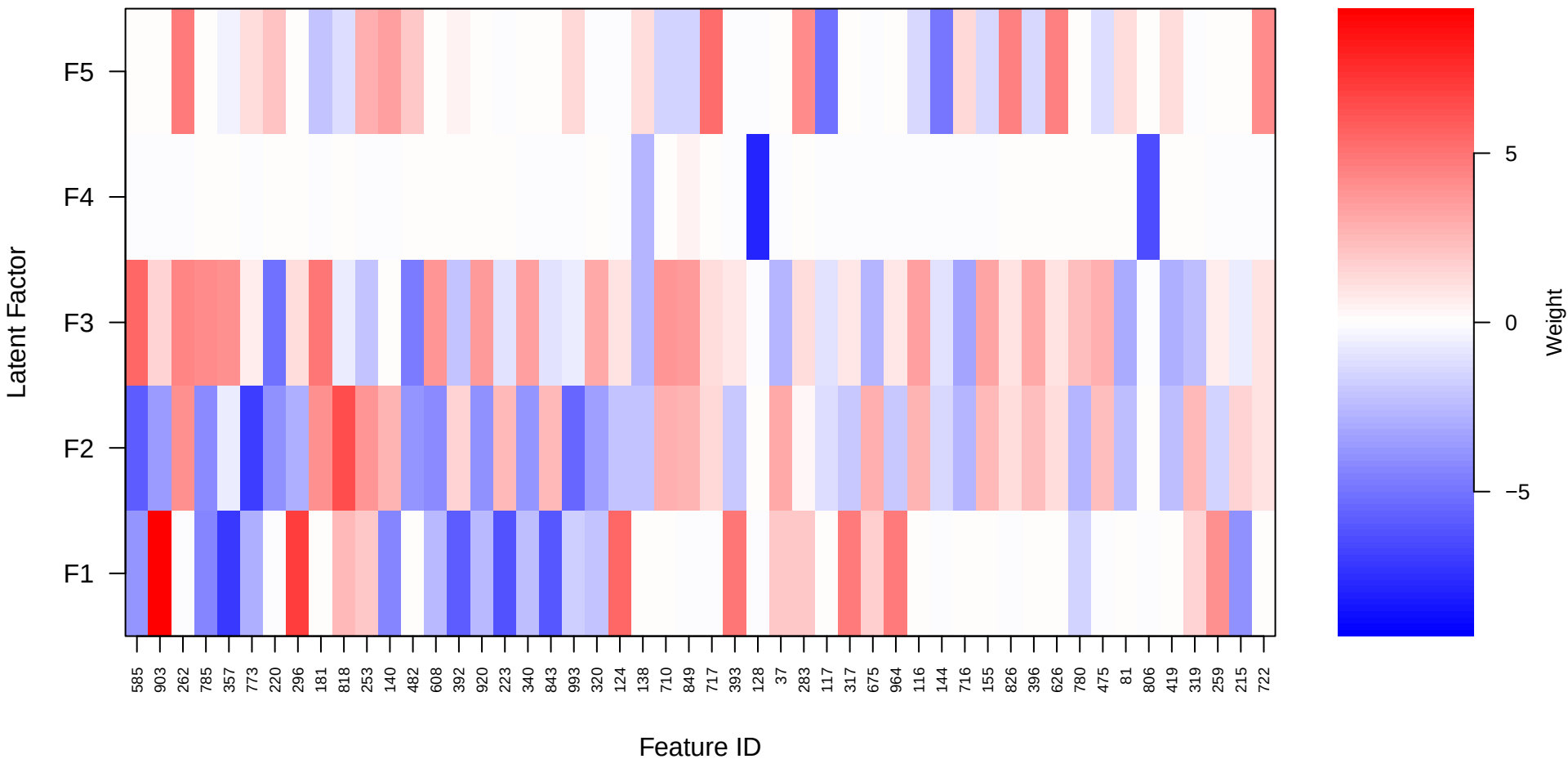
Figure 4: GEP Feature Weights (Top 50 Features)
