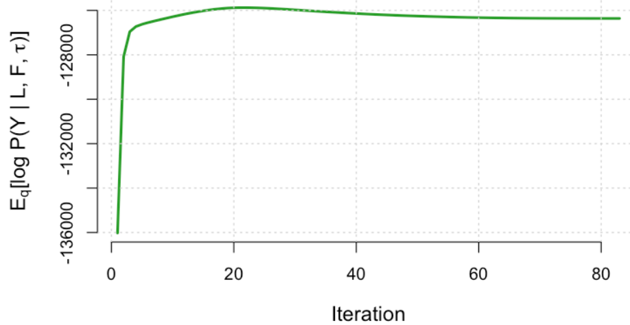
Figure 2: Genomics ELBO Proxy Across Iterations (PACA_AU_array)
