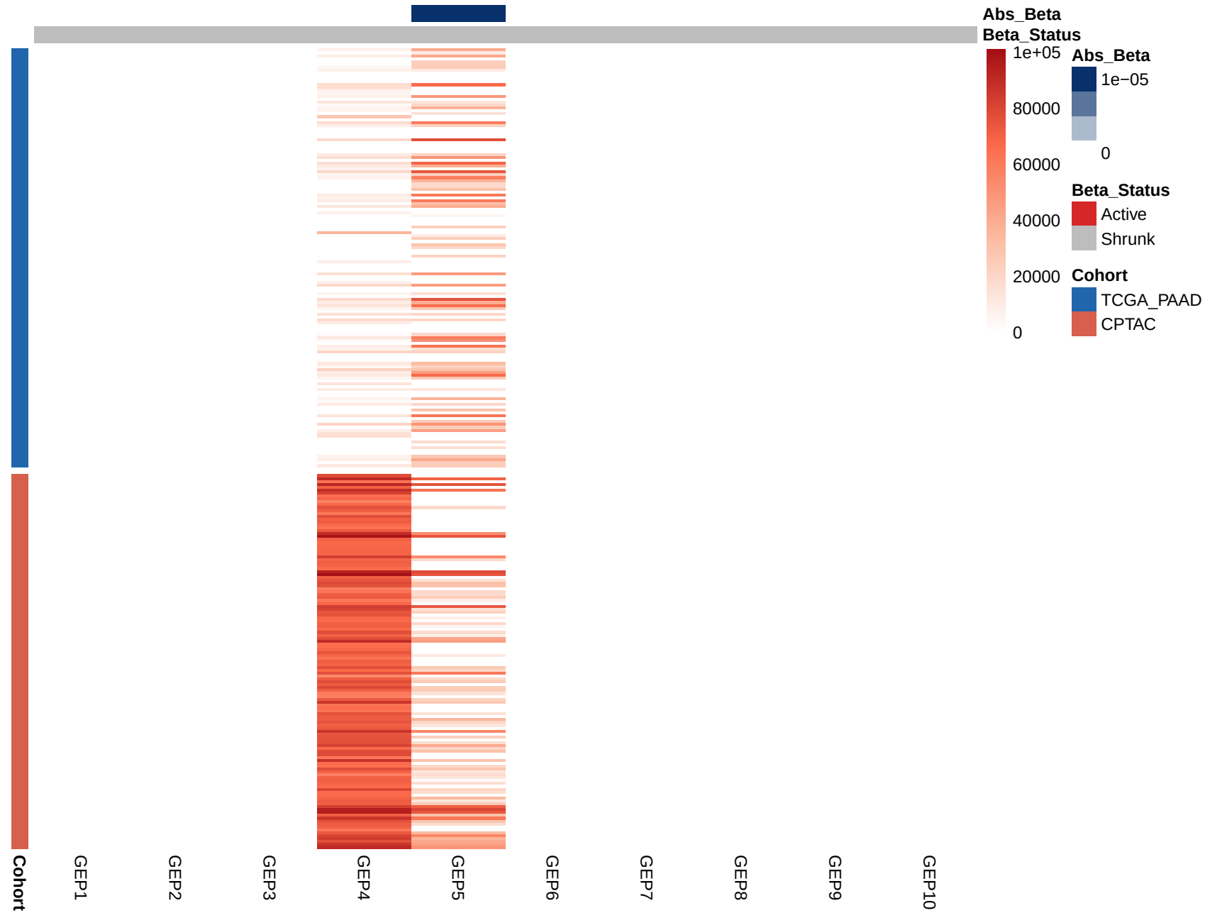
L-loading heatmap (samples by cohort) | n=273, K=10, |b|>0.05 marks 'Active'
