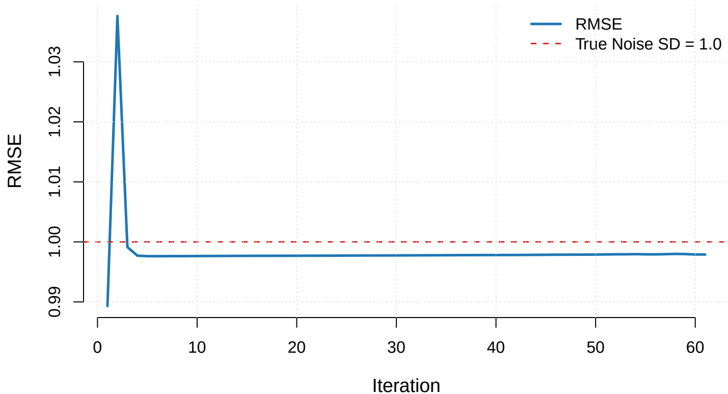
Figure 1: Reconstruction RMSE Across CAVI Iterations (Factor-Wise Modular CAVI)
