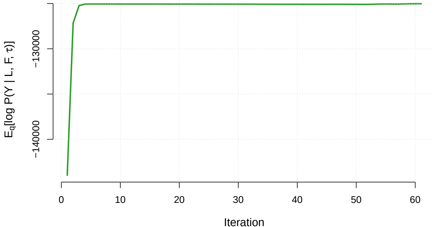
Figure 2: Genomics ELBO Proxy Across Iterations (Factor-Wise Modular CAVI)
