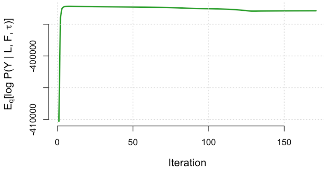
Figure 2: Genomics ELBO Proxy Across Iterations (TCGA_PAAD)
