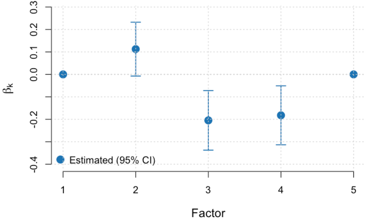
Figure 3: Estimated Survival Coefficients (95% CI) (Pooled RNA-seq: TCGA_PAAD+Dijk+PACA_AU_seq)
