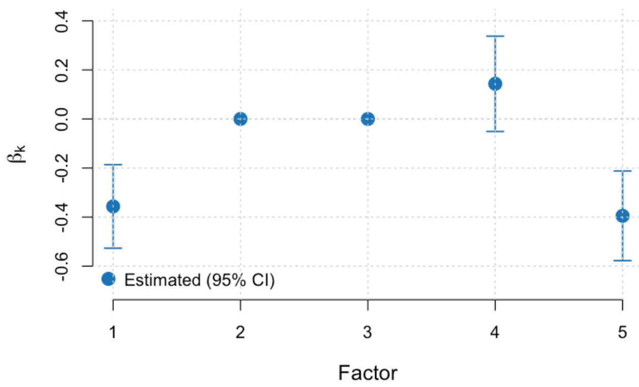
Figure 3: Estimated Survival Coefficients (95% CI) (PACA_AU_seq)
