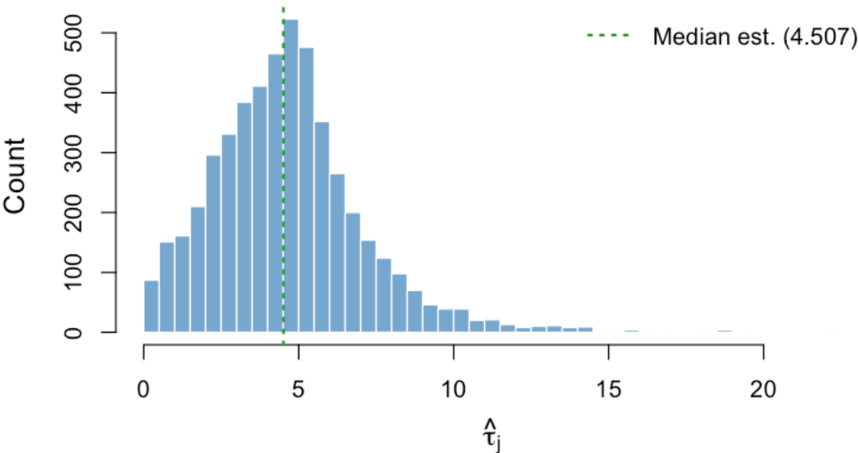
Figure 8: Estimated Feature-Specific Noise Precision (Puleo_array)
