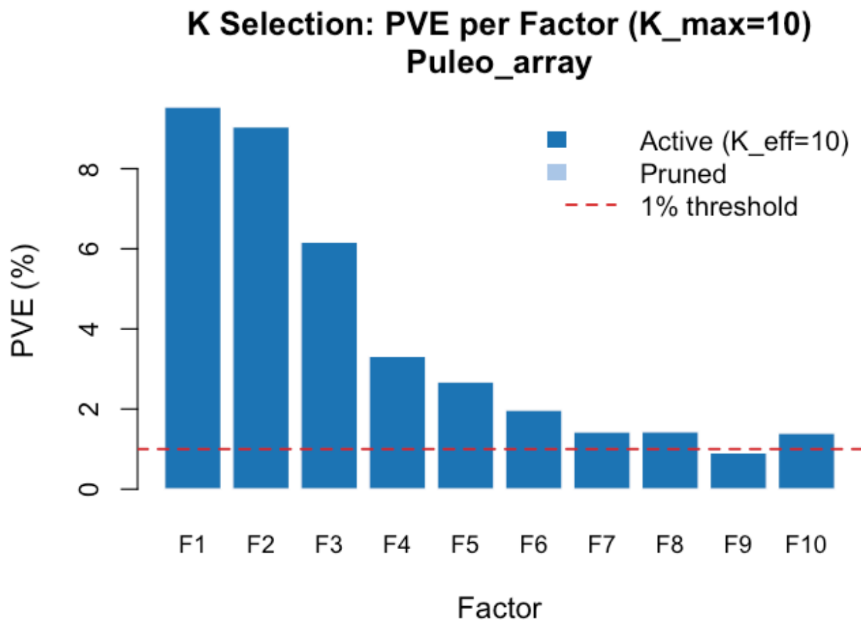
Figure 5: PVE scree plot — Puleo array ( K_{\text{eff}} = 10 )
