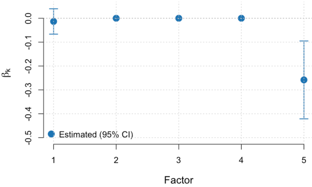
Figure 3: Estimated Survival Coefficients (95% CI) (Moffitt_GEO_array)
