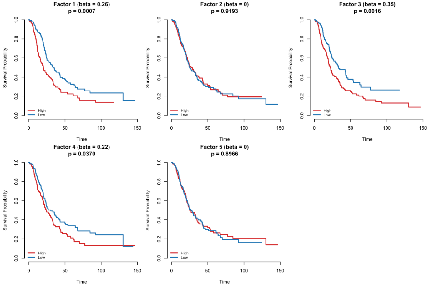
Figure 7: Kaplan-Meier survival curves by GEP activation
