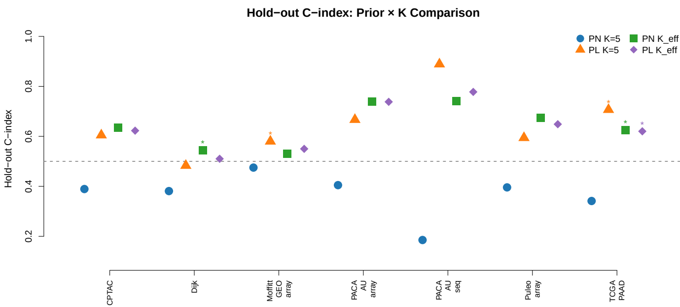
Prior × K: Scatter Plot
