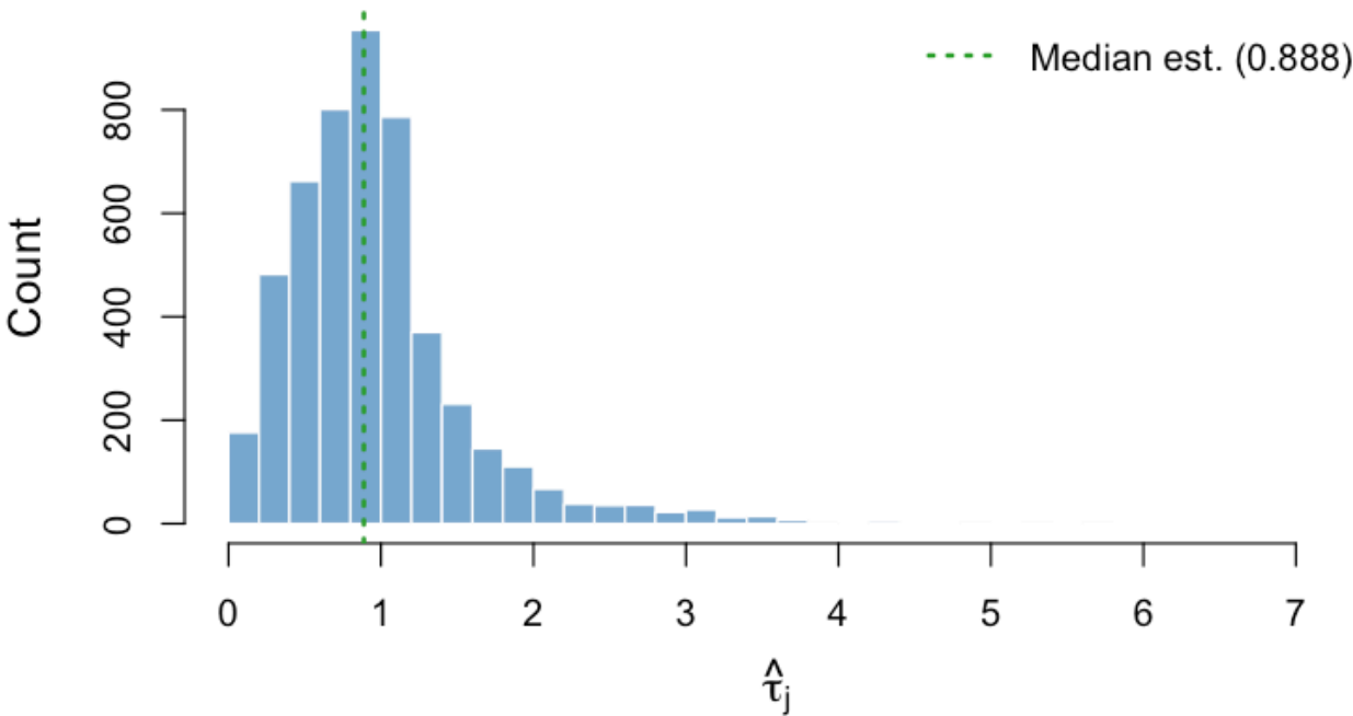
Figure 8: Estimated Feature-Specific Noise Precision (CPTAC)
