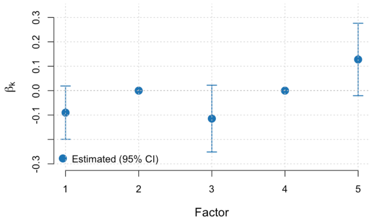
Figure 3: Estimated Survival Coefficients (95% CI) (TCGA_PAAD)
