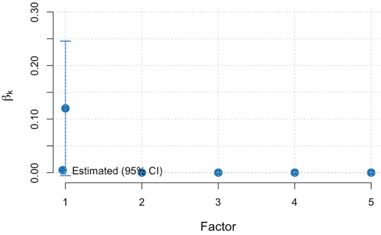
Figure 3: Estimated Survival Coefficients (95% CI) (PACA_AU_array)
