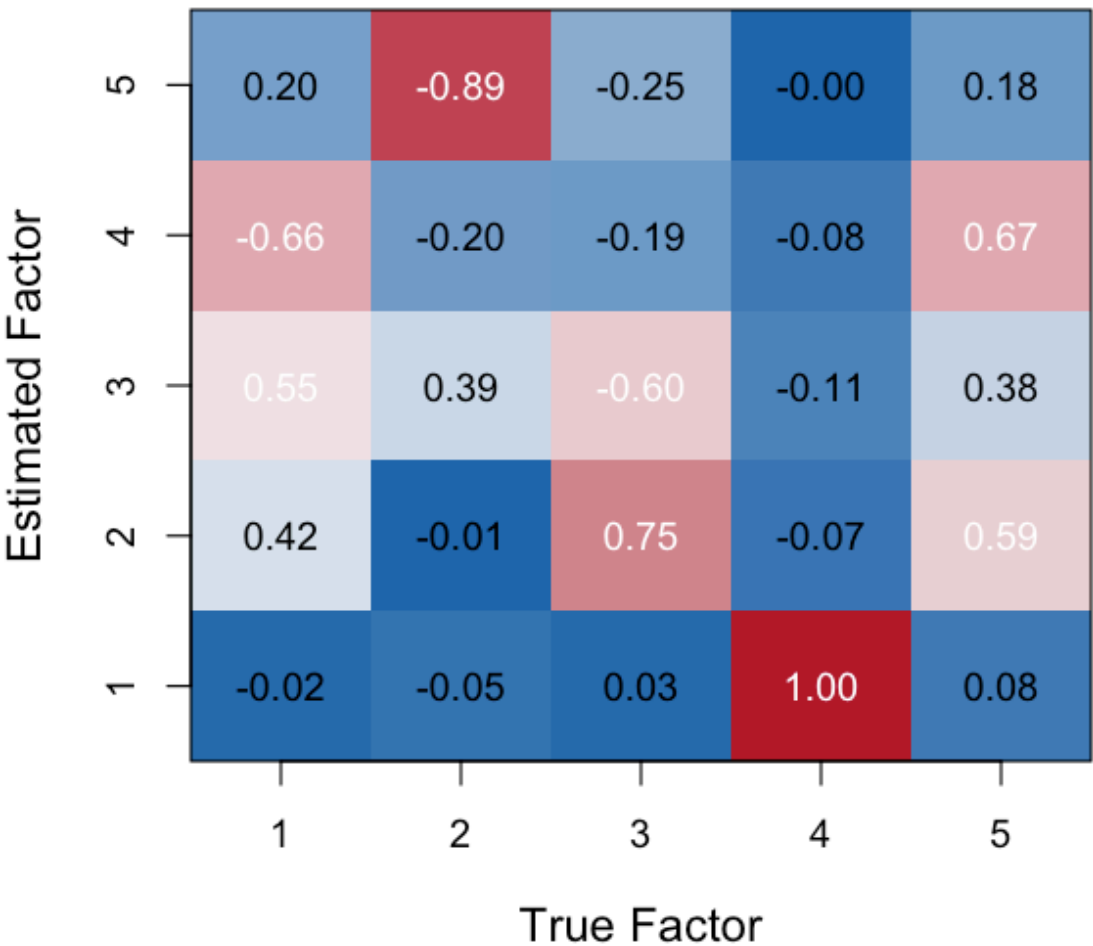
Figure 1: Loading correlations between true and estimated factors
