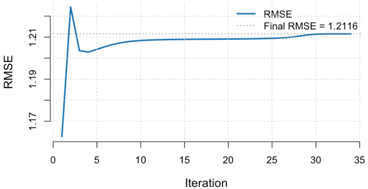
Figure 1: Reconstruction RMSE Across CAVI Iterations (CPTAC)
