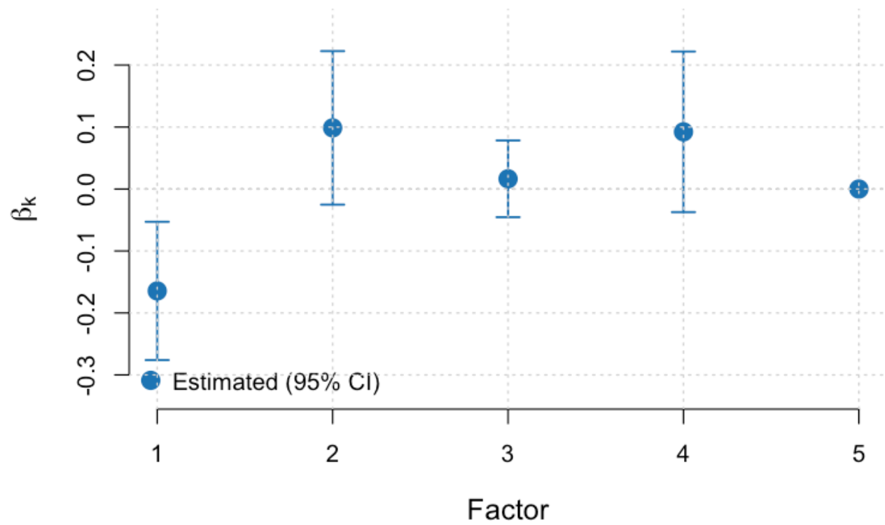
Figure 3: Estimated Survival Coefficients (95% CI) (Dijk)
