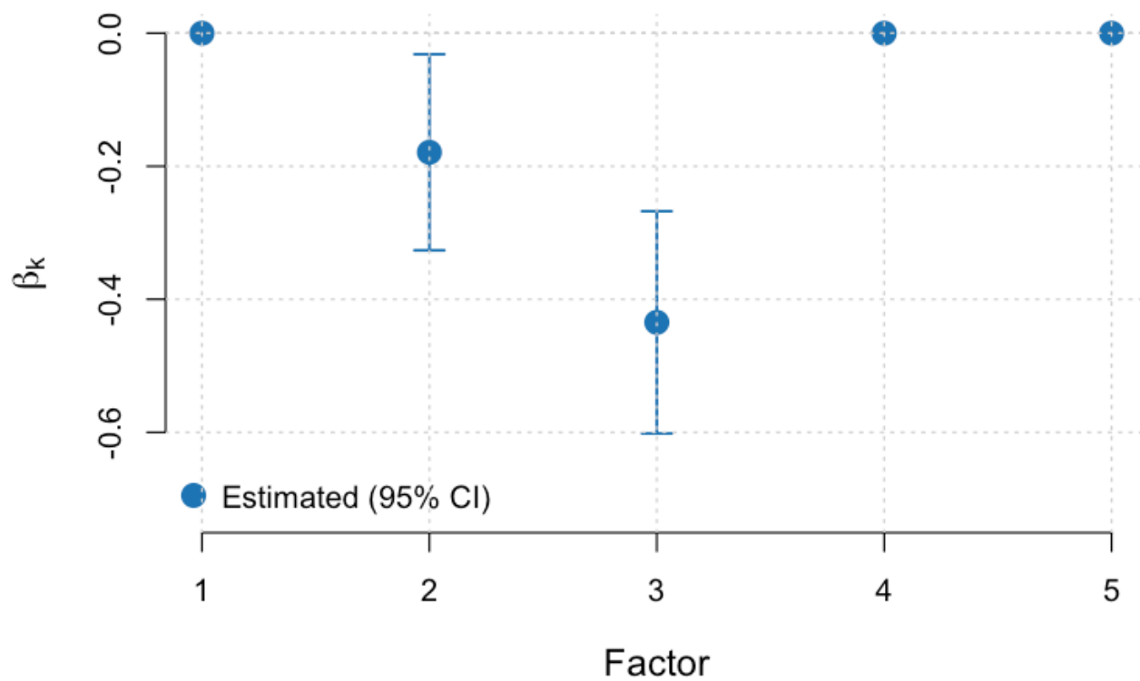
Figure 3: Estimated Survival Coefficients (95% CI) (CPTAC)
