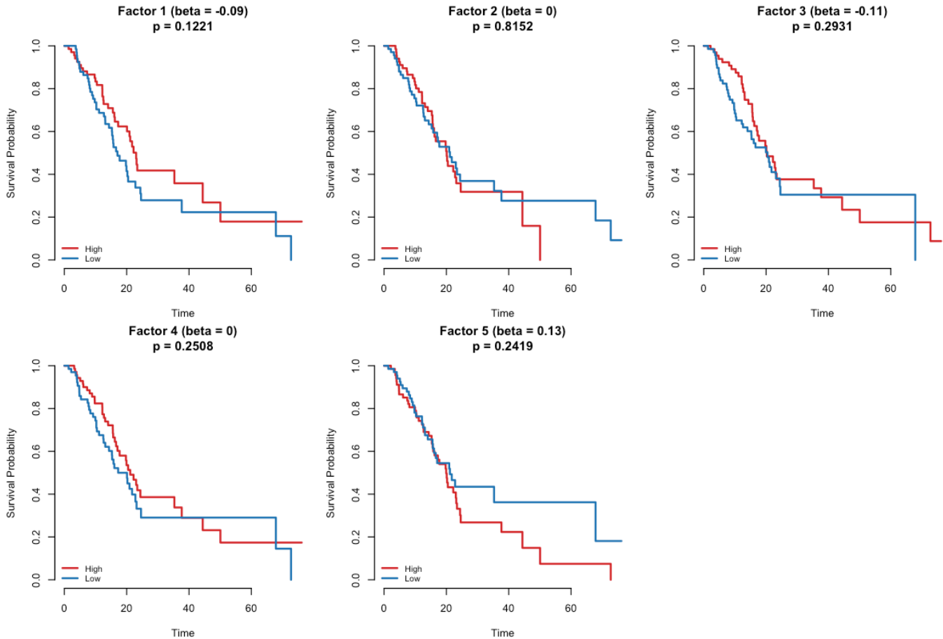
Figure 9: Kaplan-Meier survival curves by GEP activation
