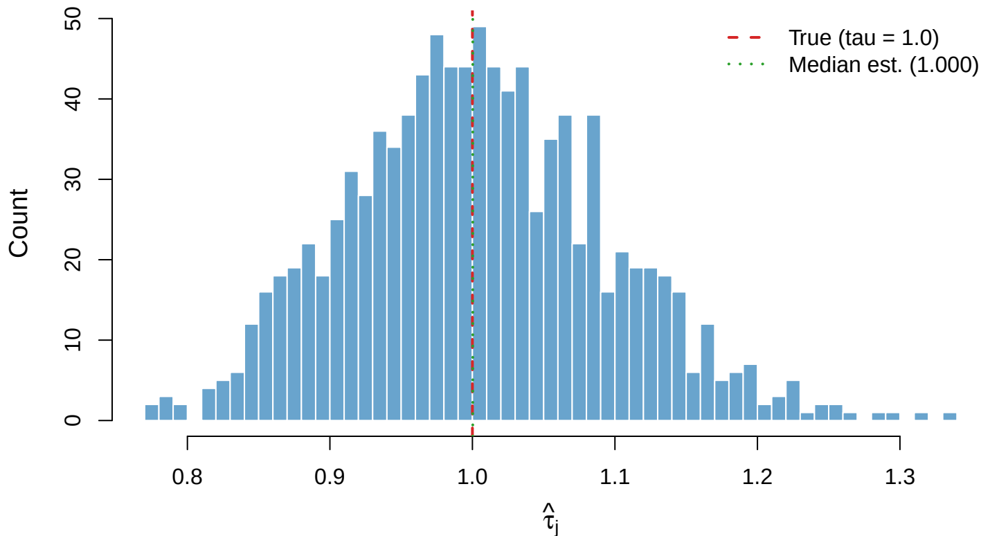
Figure 8: Estimated Feature-Specific Noise Precision (Synthetic (n=250, p=1000, K=5))
