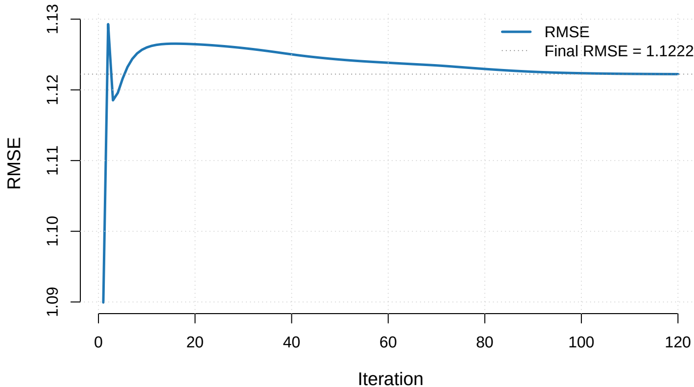
Figure 1: Reconstruction RMSE Across CAVI Iterations (Dijk)
