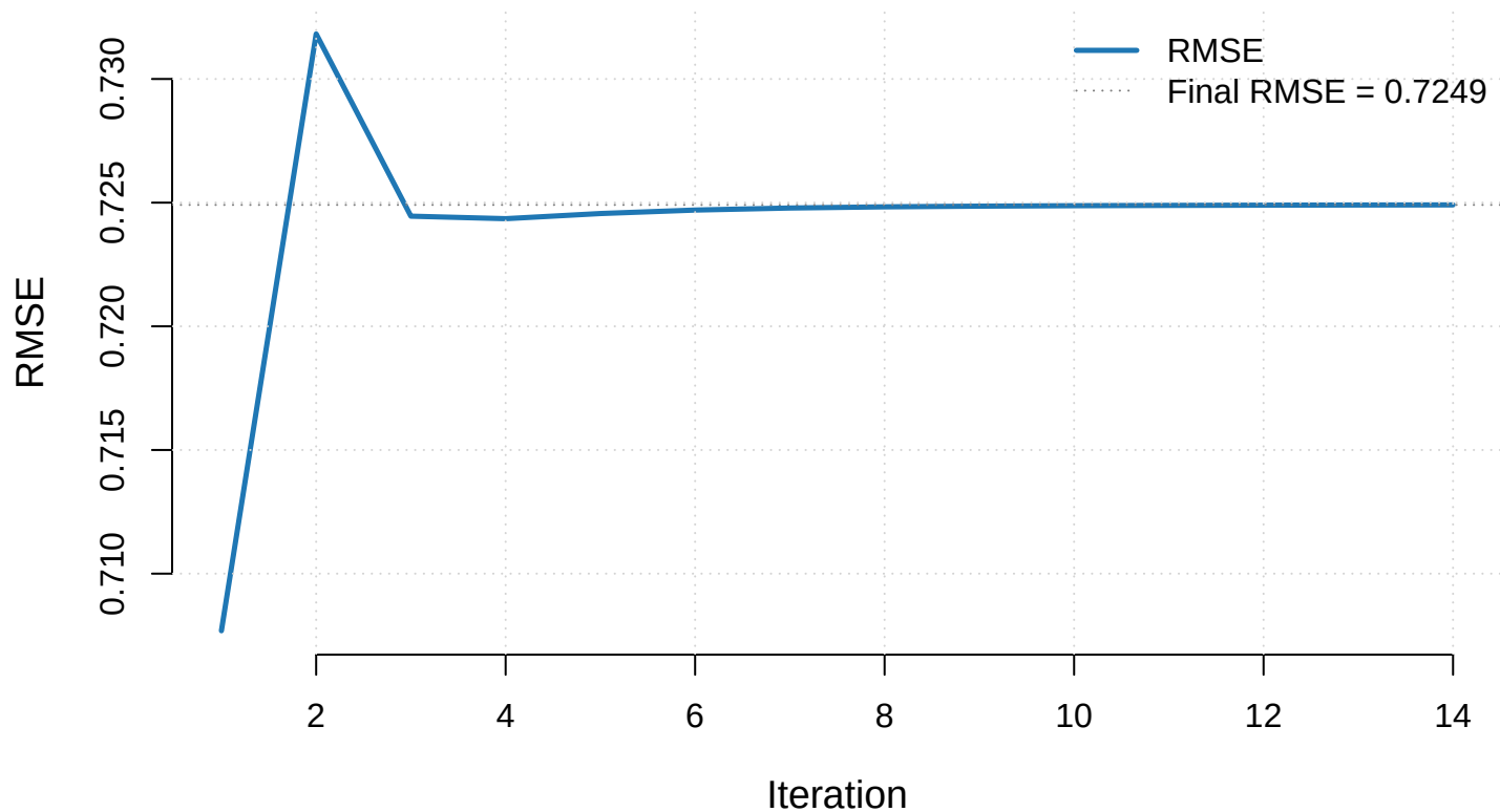
Figure 1: Reconstruction RMSE Across CAVI Iterations (Moffitt_GEO_array)
