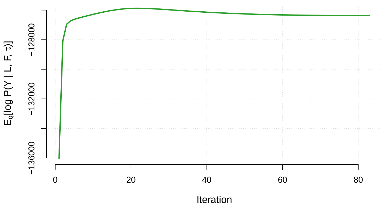
Figure 2: Genomics ELBO Proxy Across Iterations (PACA_AU_array)
