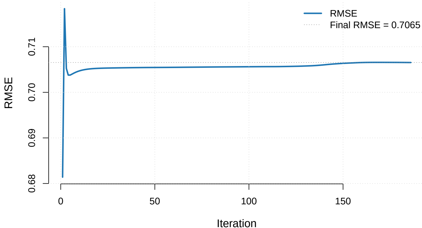
Figure 1: Reconstruction RMSE Across CAVI Iterations (PACA_AU_seq)
