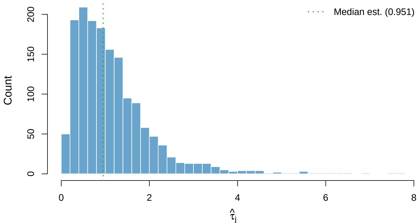
Figure 8: Estimated Feature-Specific Noise Precision (Pooled RNA-seq: TCGA_PAAD+Dijk+PACA_AU_seq)
