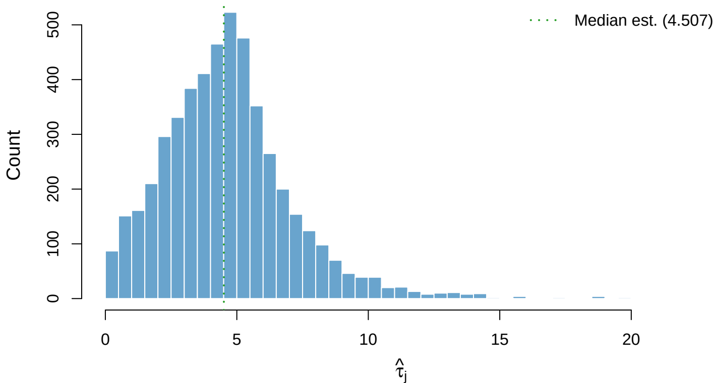
Figure 8: Estimated Feature-Specific Noise Precision (Puleo_array)
