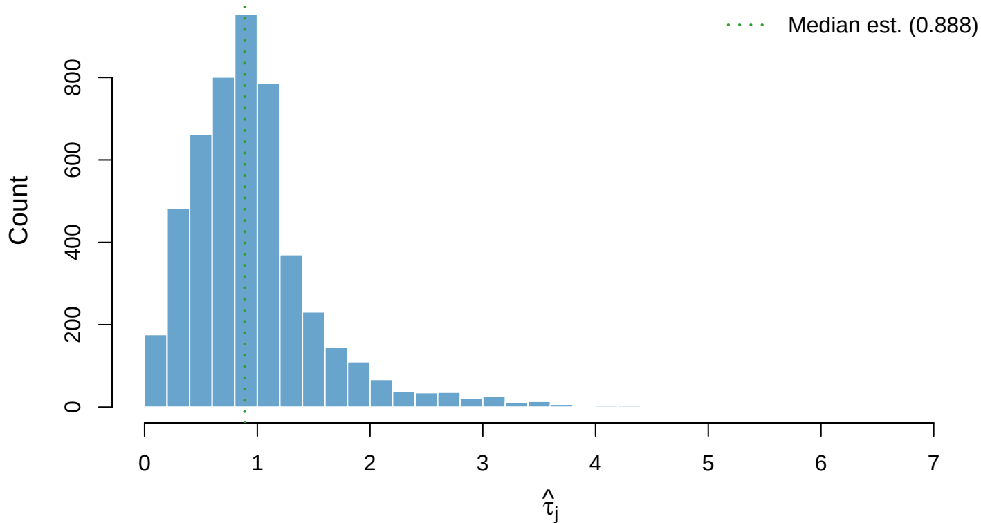
Figure 8: Estimated Feature-Specific Noise Precision (CPTAC)
