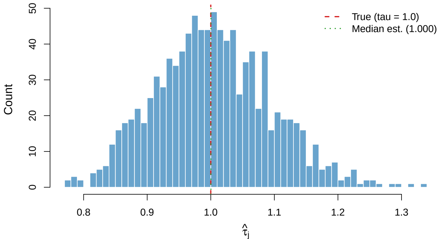
Figure 8: Estimated Feature-Specific Noise Precision (Factor-Wise Modular CAVI)
