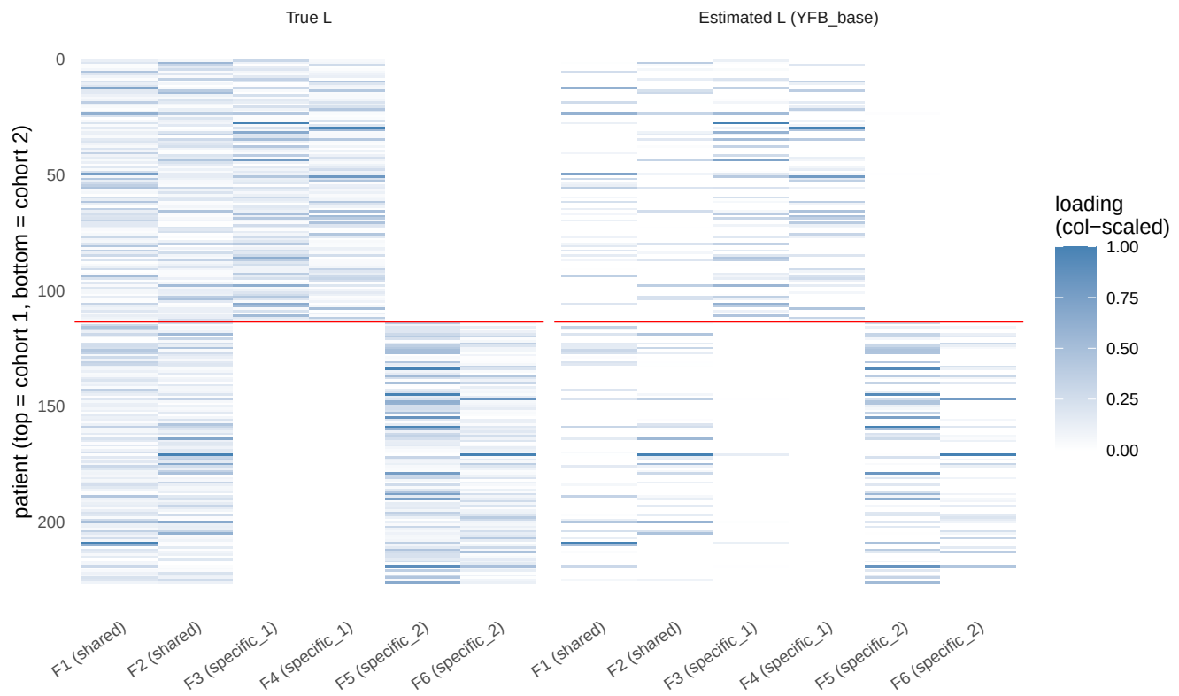
Figure 1: Patient loadings in the hybrid scenario (training patients grouped by cohort; red line = cohort boundary). Left: true loadings. Right: estimated loadings from YFB without a cohort indicator, columns reordered to the matched true factors; each column scaled to its own maximum. Shared factors (F1-F2) load across BOTH cohorts; cohort-1-specific factors (F3-F4) light up only the top block, cohort-2-specific (F5-F6) only the bottom. The estimate reproduces the true block-sparse pattern — the model identifies shared vs. cohort-private factors with no indicator columns.
