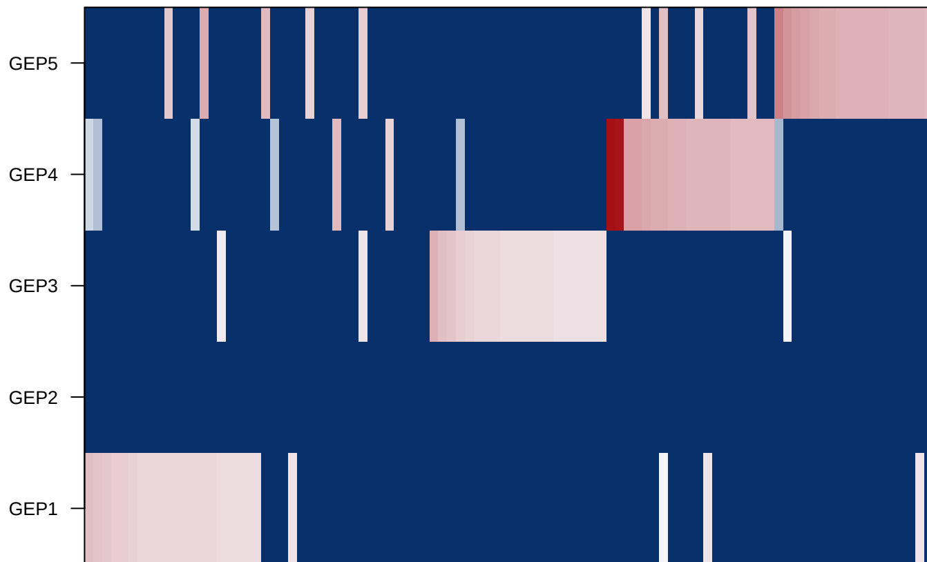
GEP Loading Heatmap (matched factors)
