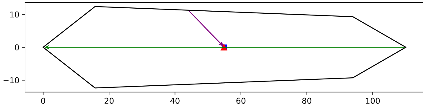
optical probe paths (frozen ray_to_target, 632.8 nm)
