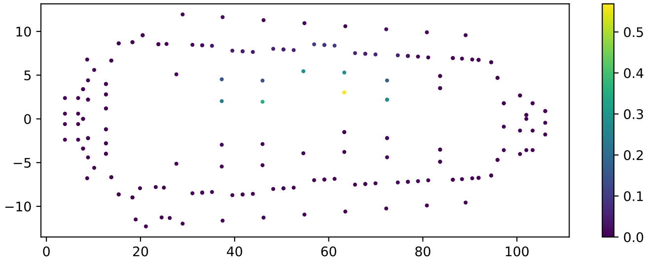
D5 electric-energy density, static 10 V electrodes (solved piezo)
