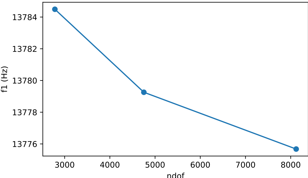
mesh convergence, first elastic mode (ideal)
