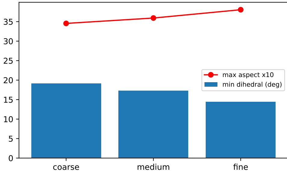
mesh quality by level
