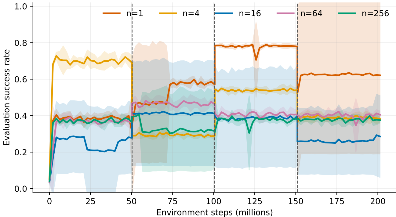
Continual learning across four topology distributions
