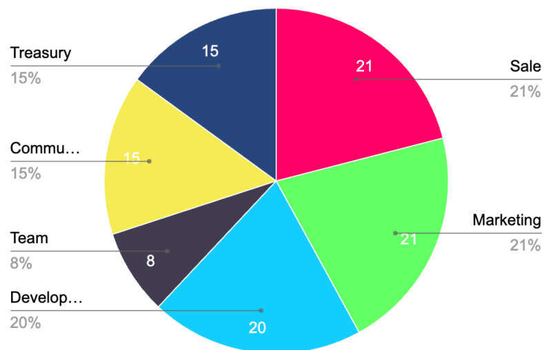
Token Allocation
