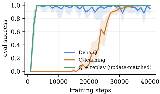
(a) Sample efficiency, HOME A
