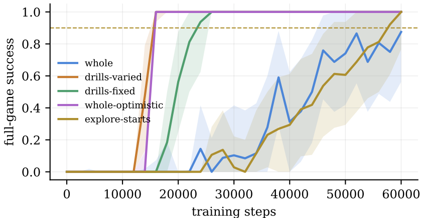
Reverse start-state curriculum
