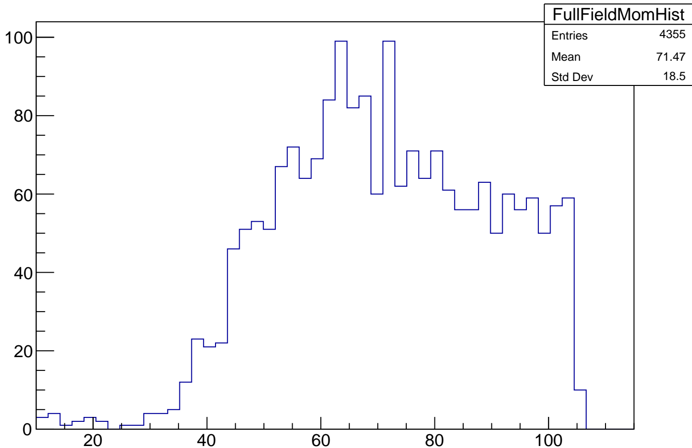
Momentum (MeV/c) of a Sample Dataset at Full DS Solenoid Magnetic Field
