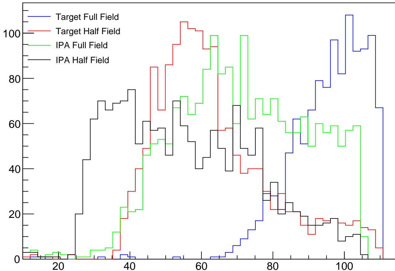
Momentum (MeV/c) Comparison For Target and IPA Stops at Full and Half Field Strengths for the DS
