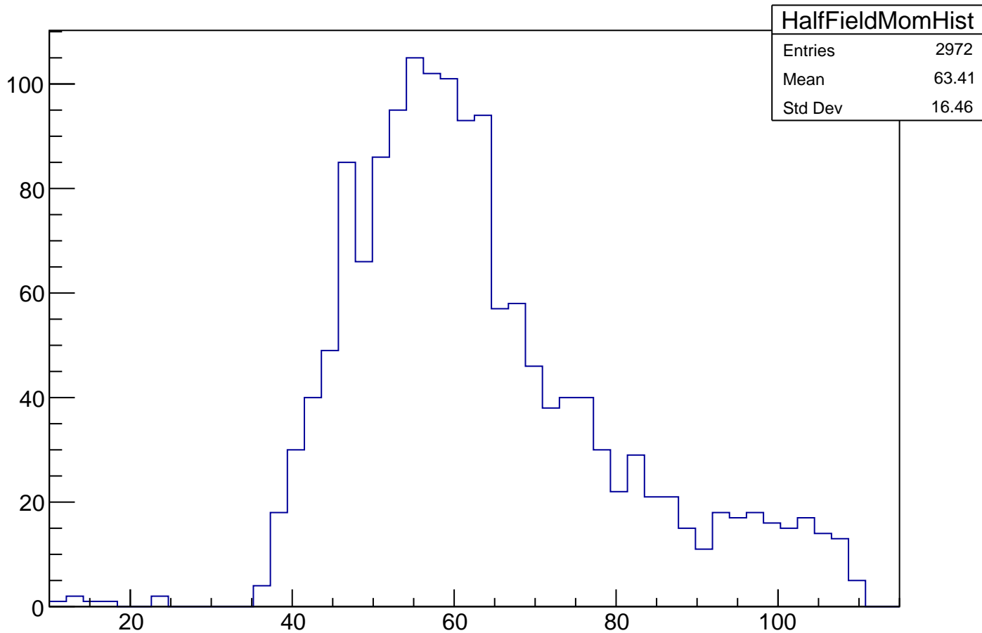
Momentum (MeV/c) of a Sample Dataset at Half DS Solenoid Magnetic Field
