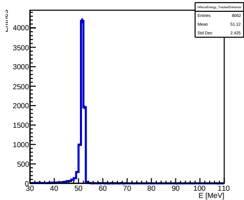
B2BCeEndpointDiffEnergy Reco Energy at Tracker Entrance (TT_Front)
