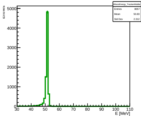
B2BCeEndpointDiffEnergy Reco Energy at Tracker Middle (TT_Mid)
