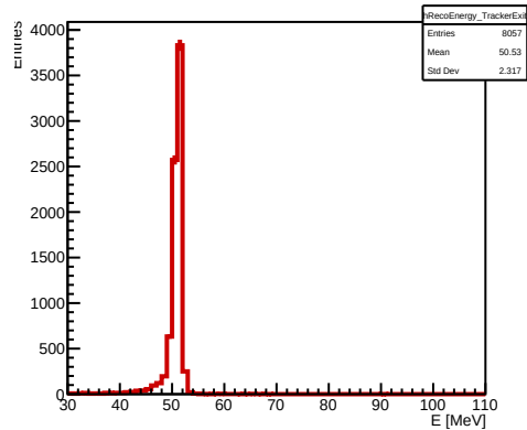
B2BCeEndpointDiffEnergy Reco Energy at Tracker Exit (TT_Back)
